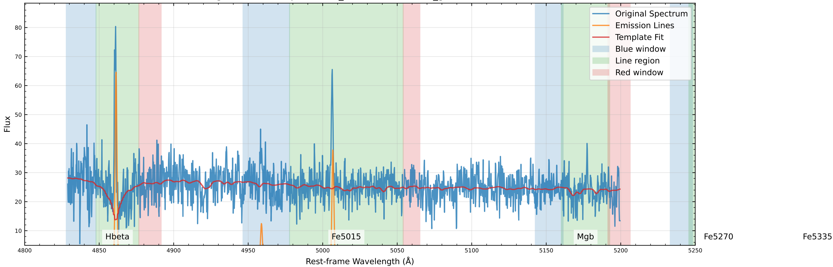
Original Data Comparison (v_star=-54.7 km/s, v_gas=-34.1 km/s)
