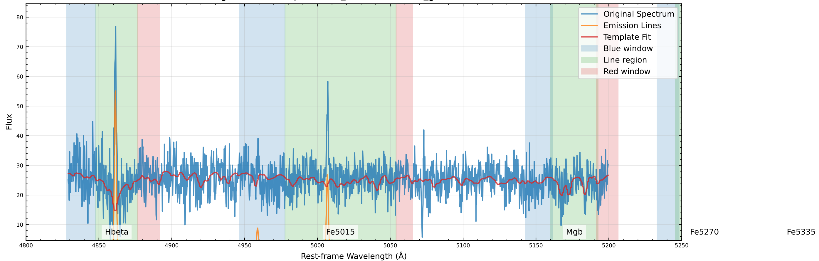
Original Data Comparison (v_star=1.1 km/s, v_gas=-0.2 km/s)
