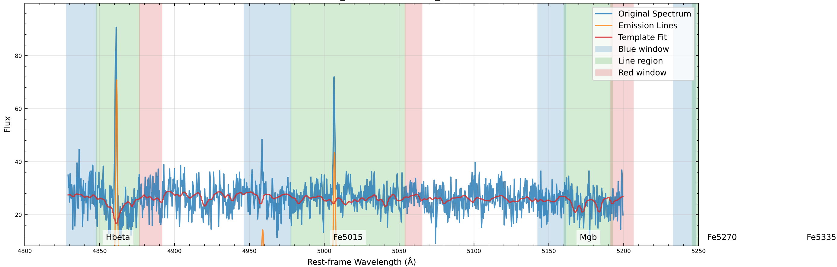
Original Data Comparison (v_star=-20.7 km/s, v_gas=-26.2 km/s)
