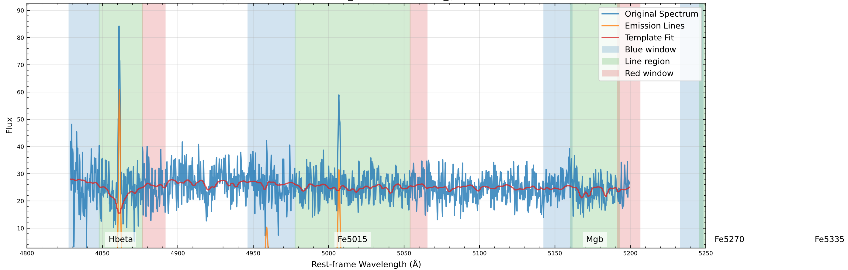
Original Data Comparison (v_star=-20.7 km/s, v_gas=-5.2 km/s)
