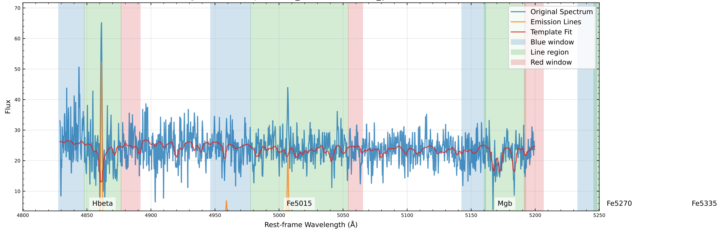
Original Data Comparison (v_star=-32.2 km/s, v_gas=-3.9 km/s)
