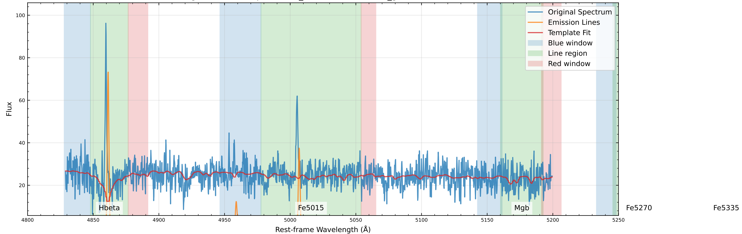
Original Data Comparison (v_star=-101.3 km/s, v_gas=-101.8 km/s)
