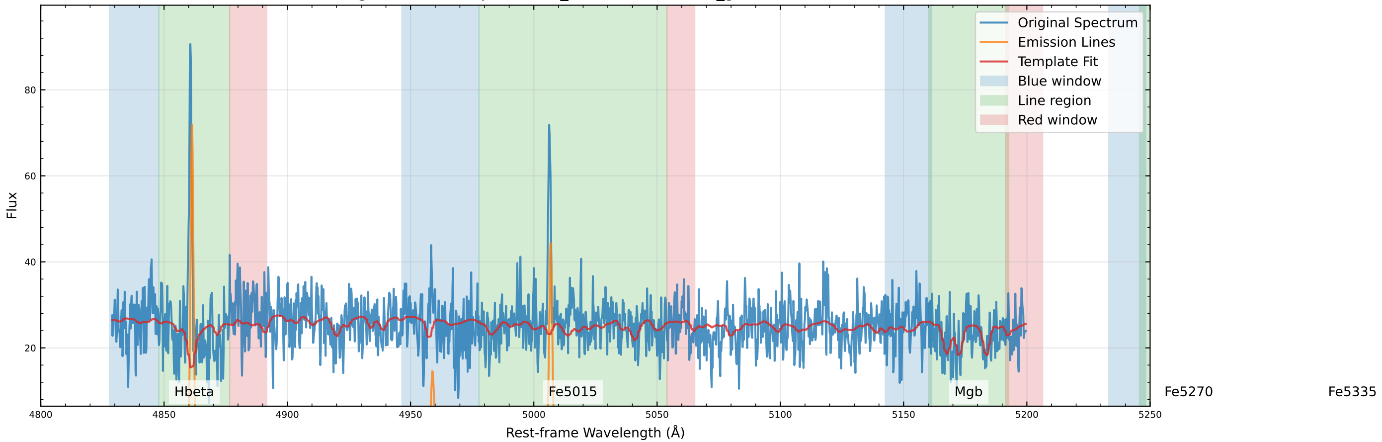
Original Data Comparison (v_star=-35.8 km/s, v_gas=-38.1 km/s)
