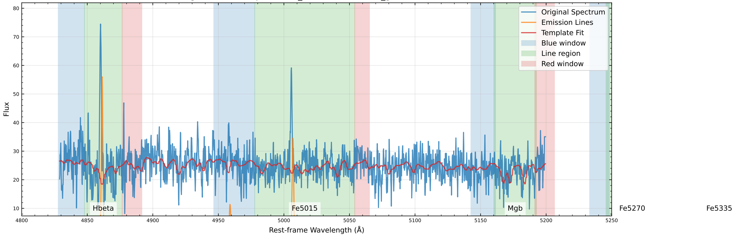
Original Data Comparison (v_star=-88.1 km/s, v_gas=-73.3 km/s)
