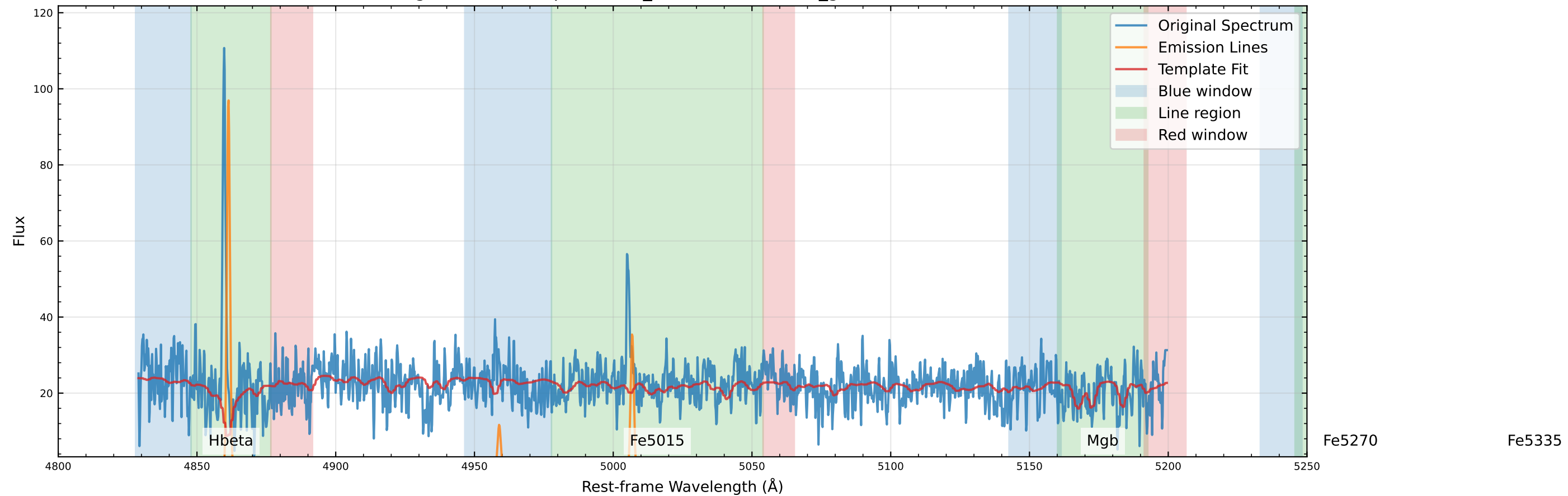
Original Data Comparison (v_star=-76.3 km/s, v_gas=-95.2 km/s)
