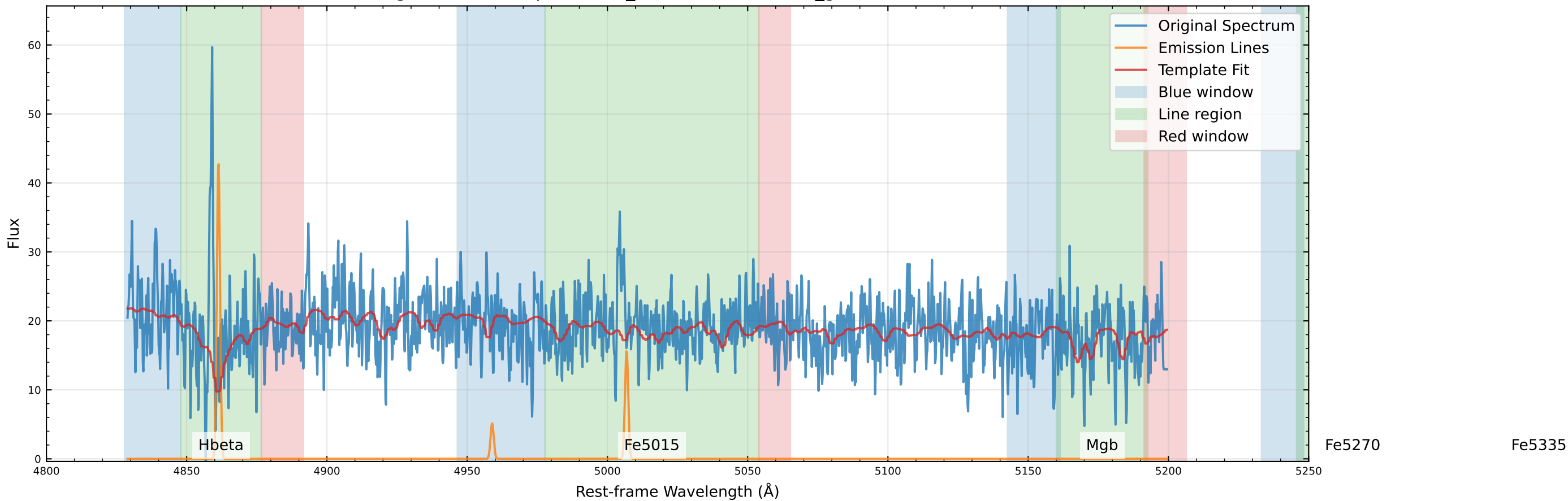
Original Data Comparison (v_star=-155.2 km/s, v_gas=-153.7 km/s)
