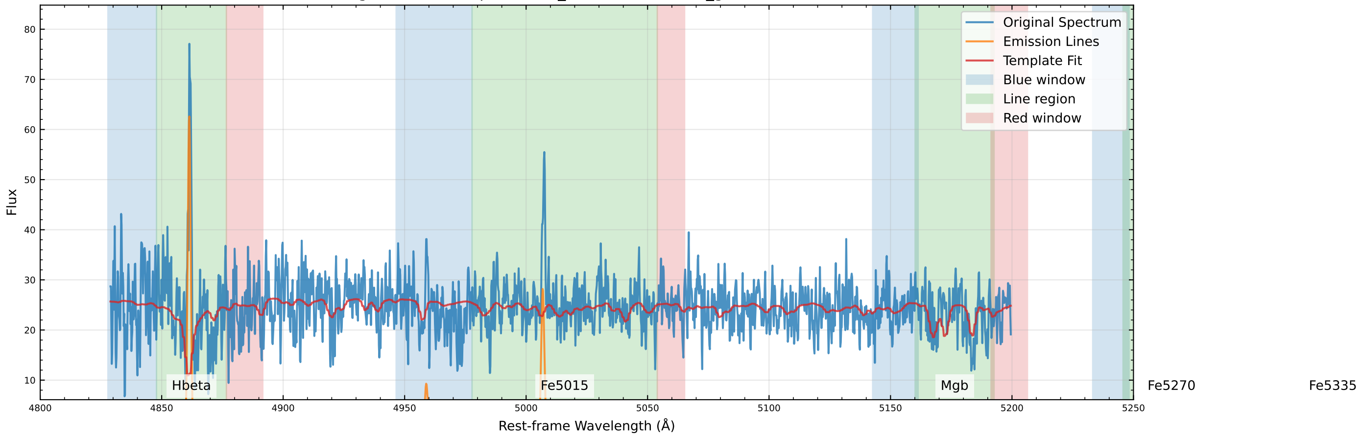
Original Data Comparison (v_star=26.7 km/s, v_gas=17.3 km/s)
