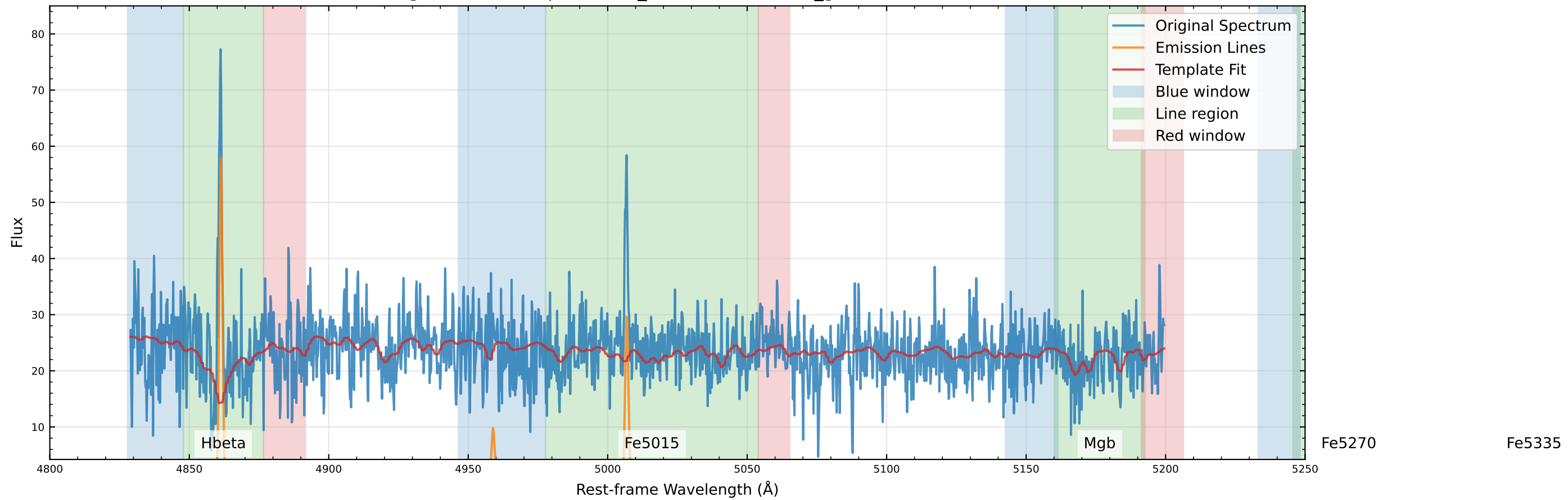
Original Data Comparison (v_star=-19.2 km/s, v_gas=-14.2 km/s)
