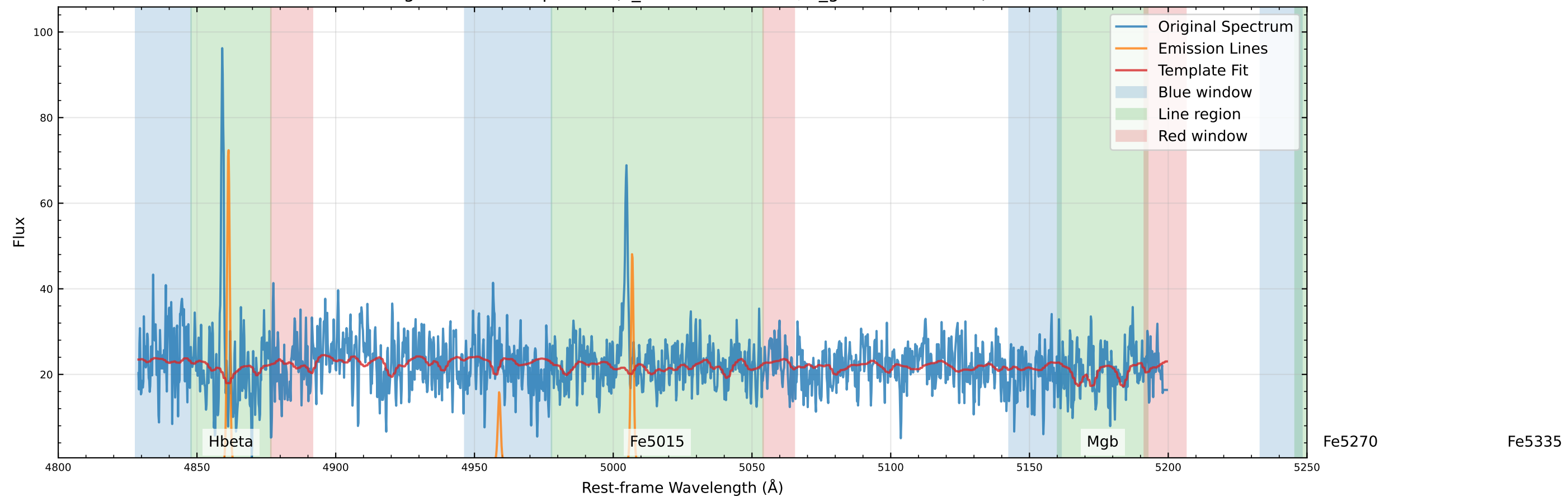
Original Data Comparison (v_star=-150.9 km/s, v_gas=-133.2 km/s)
