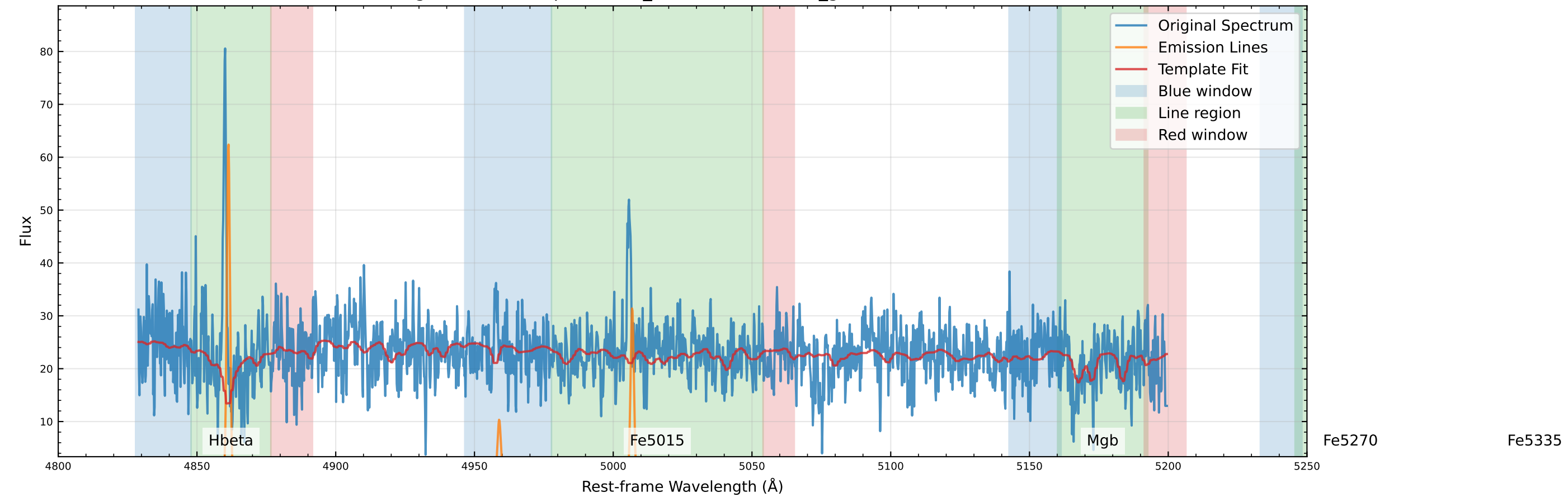
Original Data Comparison (v_star=-55.8 km/s, v_gas=-78.8 km/s)
