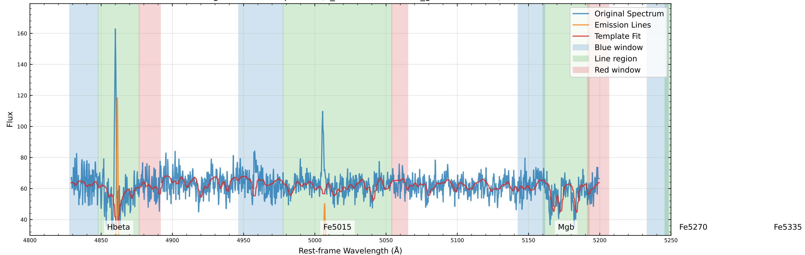
Original Data Comparison (v_star=-83.9 km/s, v_gas=-83.2 km/s)
