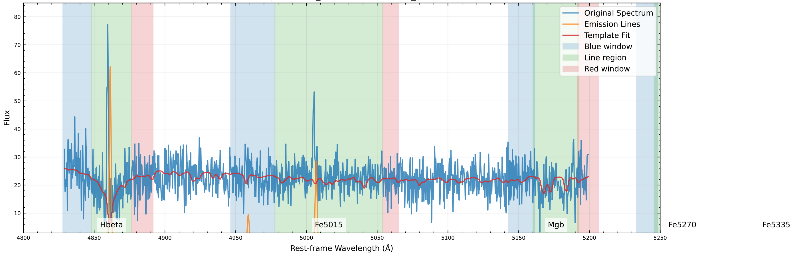
Original Data Comparison (v_star=-123.1 km/s, v_gas=-109.6 km/s)
