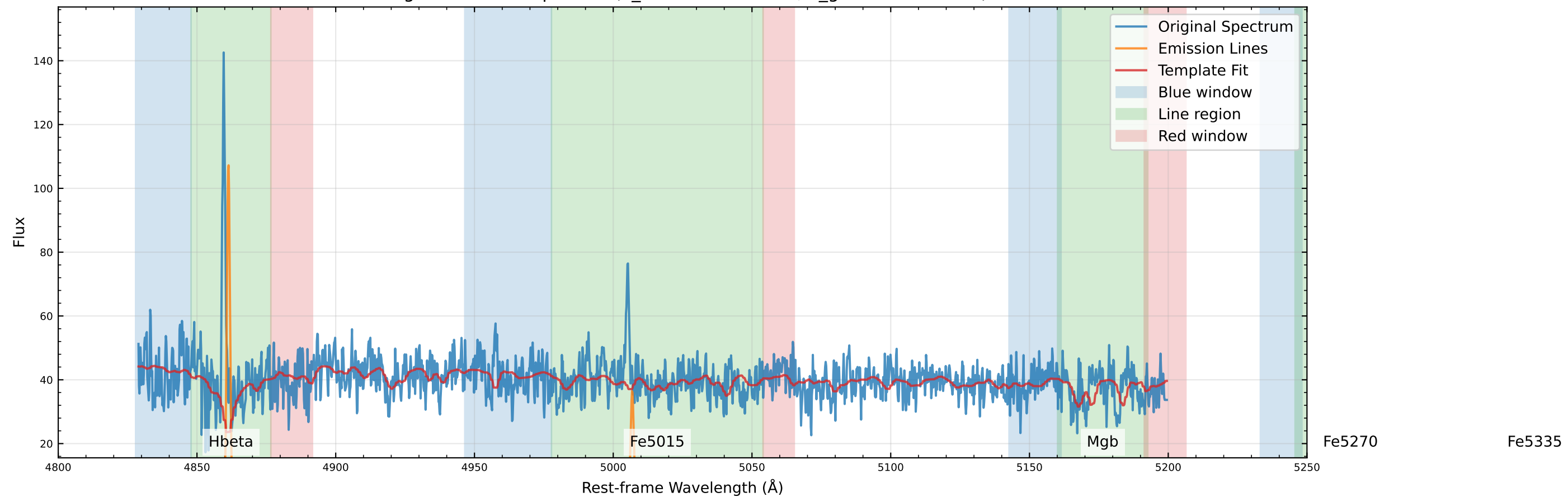
Original Data Comparison (v_star=-100.7 km/s, v_gas=-102.9 km/s)
