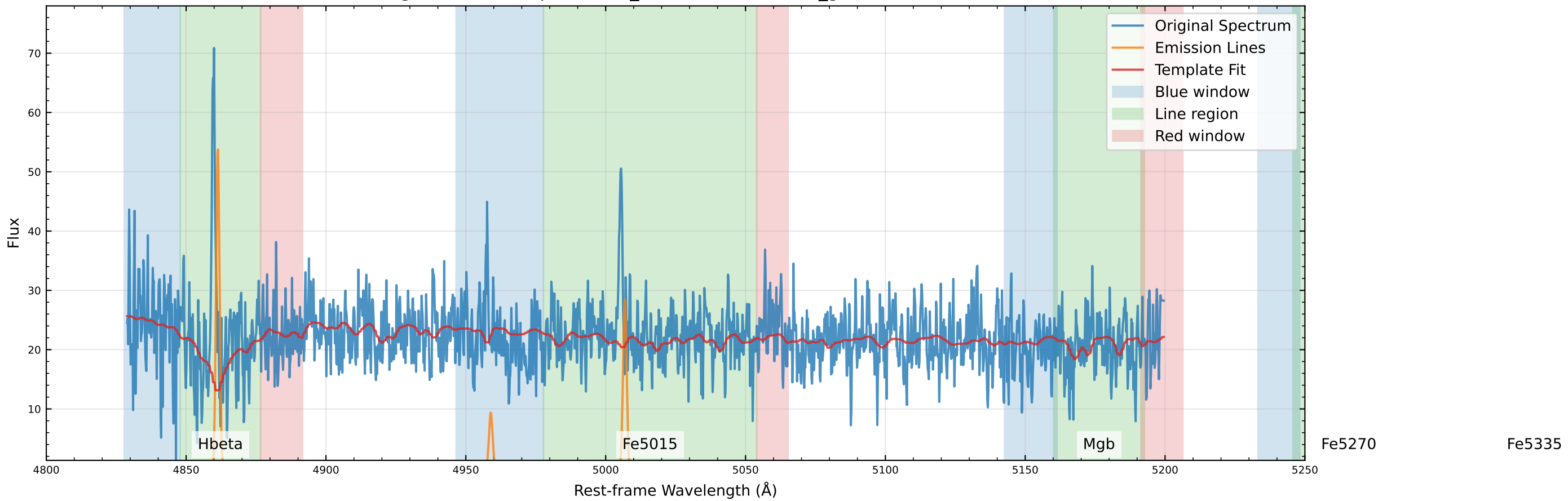
Original Data Comparison (v_star=-113.7 km/s, v_gas=-94.8 km/s)
