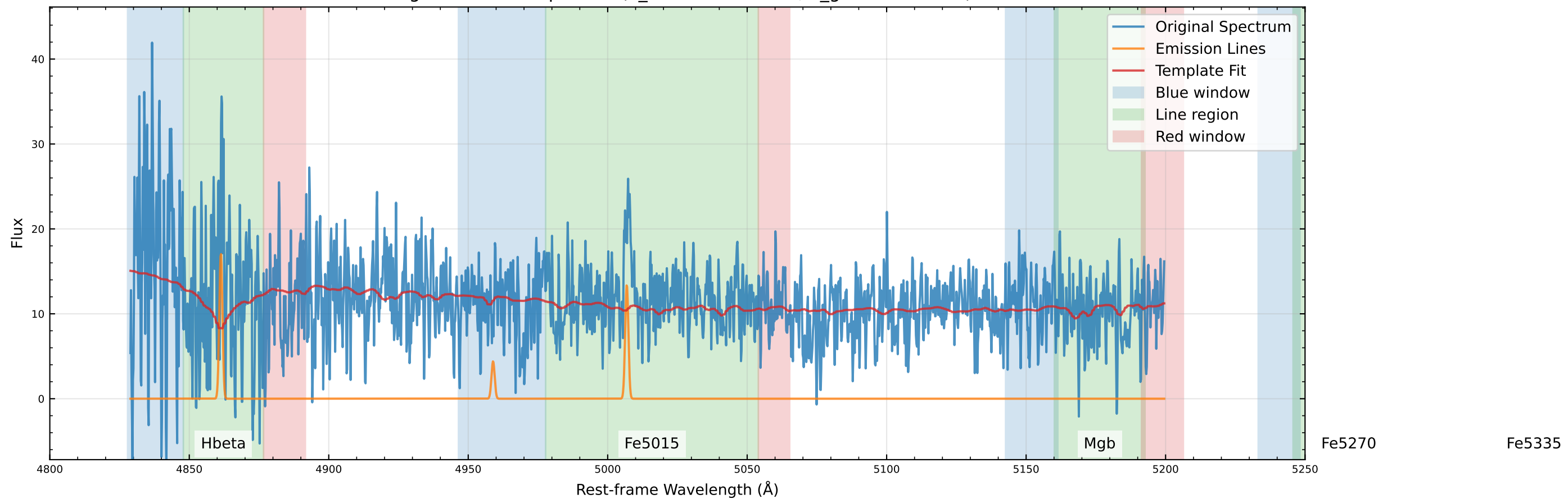
Original Data Comparison (v_star=199.9 km/s, v_gas=27.3 km/s)
