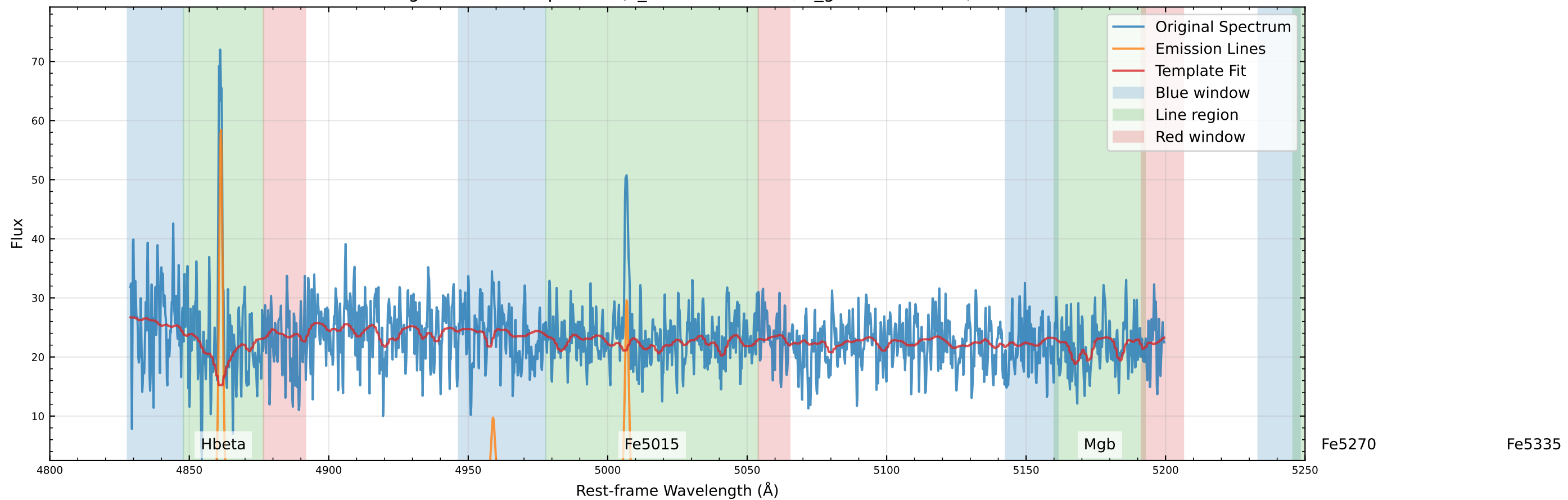
Original Data Comparison (v_star=-35.2 km/s, v_gas=-12.1 km/s)
