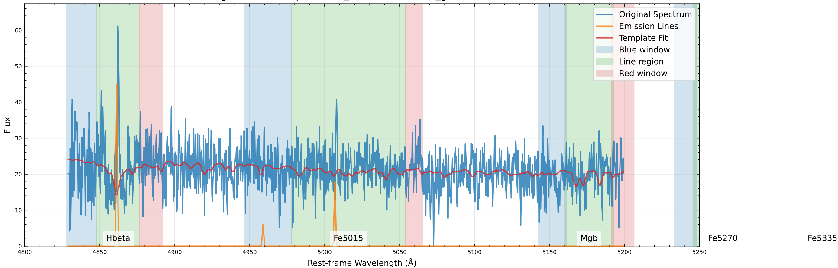
Original Data Comparison (v_star=89.5 km/s, v_gas=59.3 km/s)
