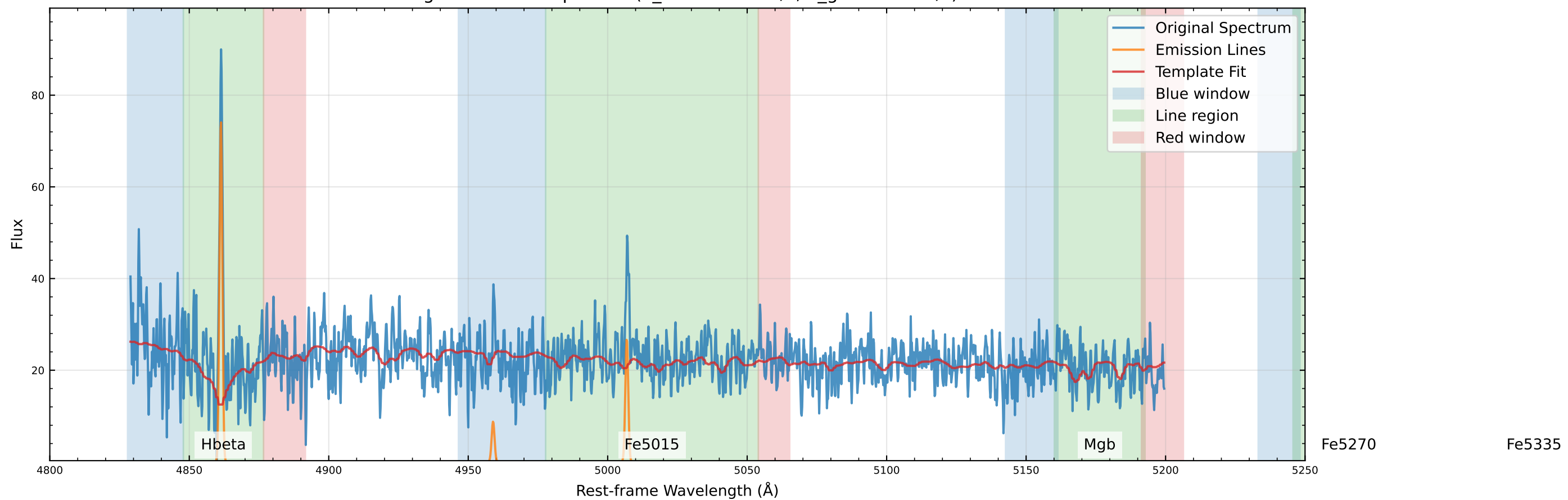
Original Data Comparison ( v_{\text{star}}=-8.5 km/s, v_{\text{gas}}=4.6 km/s)
