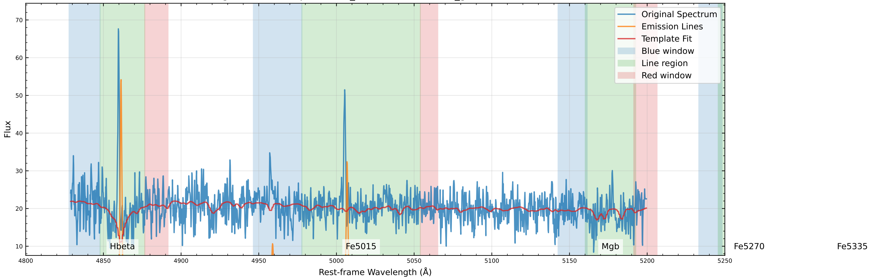
Original Data Comparison (v_star=-106.3 km/s, v_gas=-96.0 km/s)
