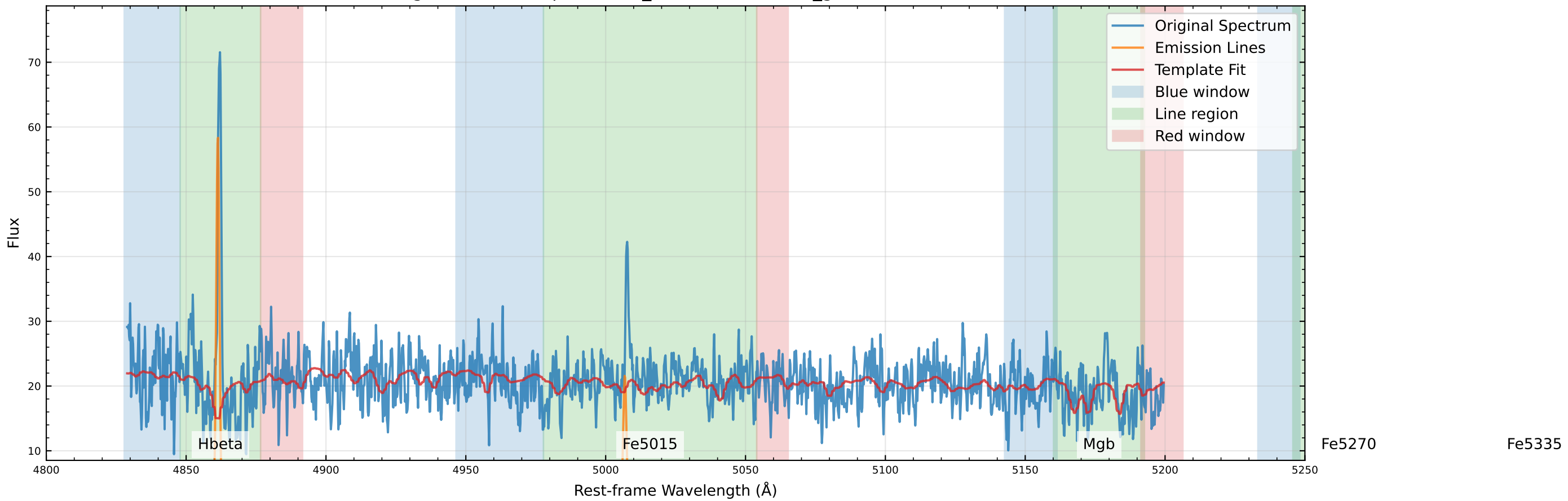
Original Data Comparison (v_star=66.7 km/s, v_gas=39.3 km/s)
