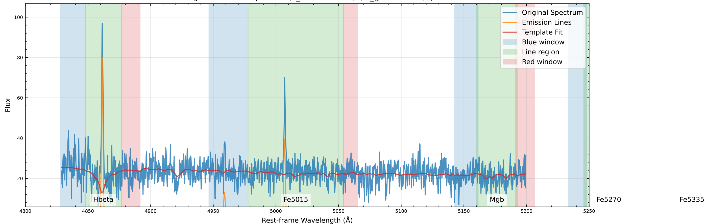
Original Data Comparison (v_star=-3.9 km/s, v_gas=7.8 km/s)
