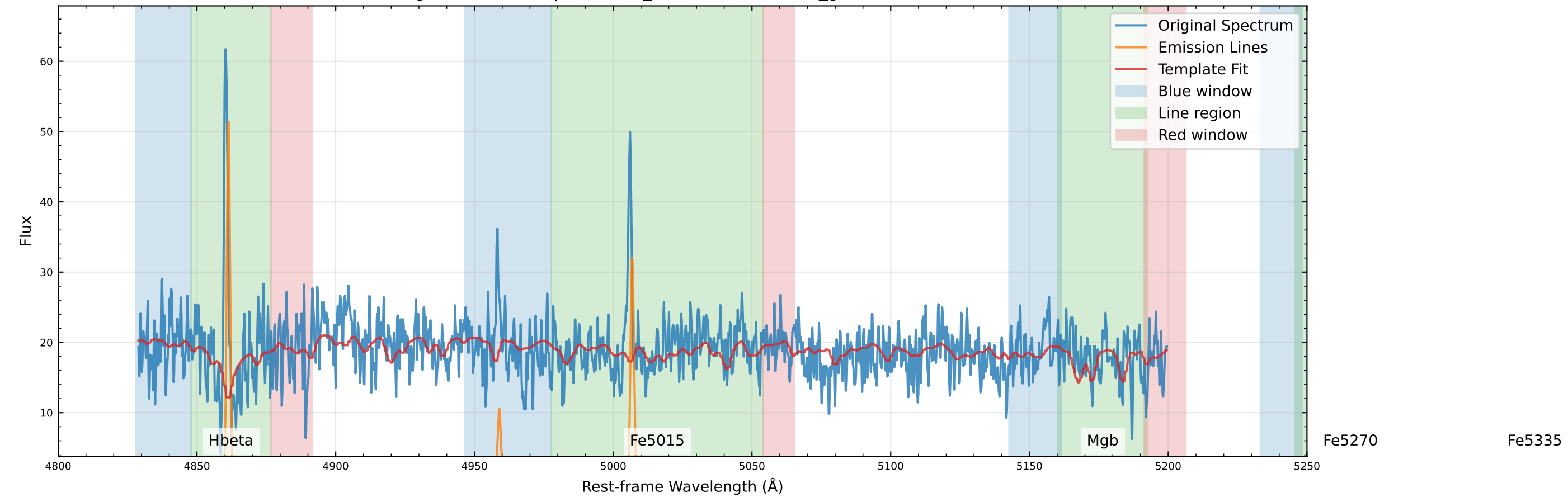
Original Data Comparison (v_star=-32.9 km/s, v_gas=-54.7 km/s)
