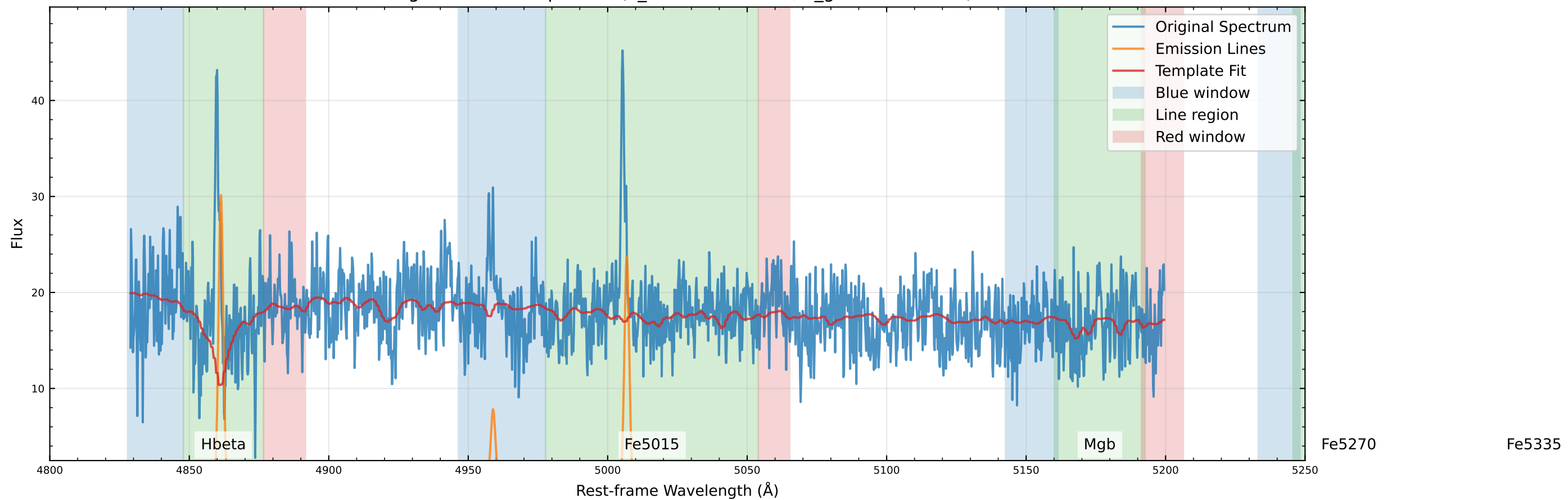
Original Data Comparison (v_star=-56.1 km/s, v_gas=-82.6 km/s)
