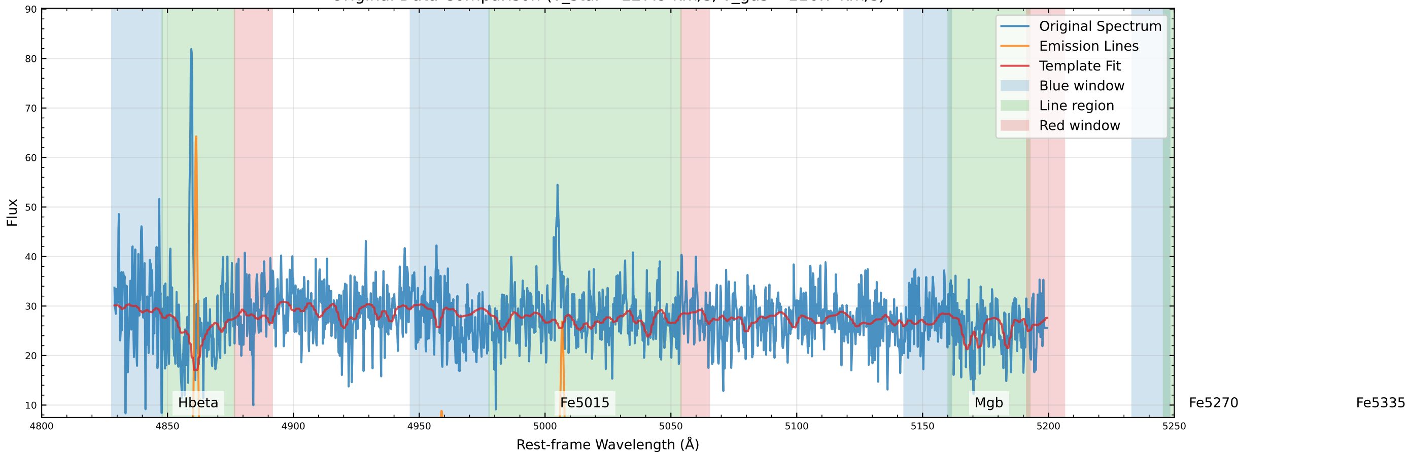
Original Data Comparison (v_star=-127.9 km/s, v_gas=-116.7 km/s)
