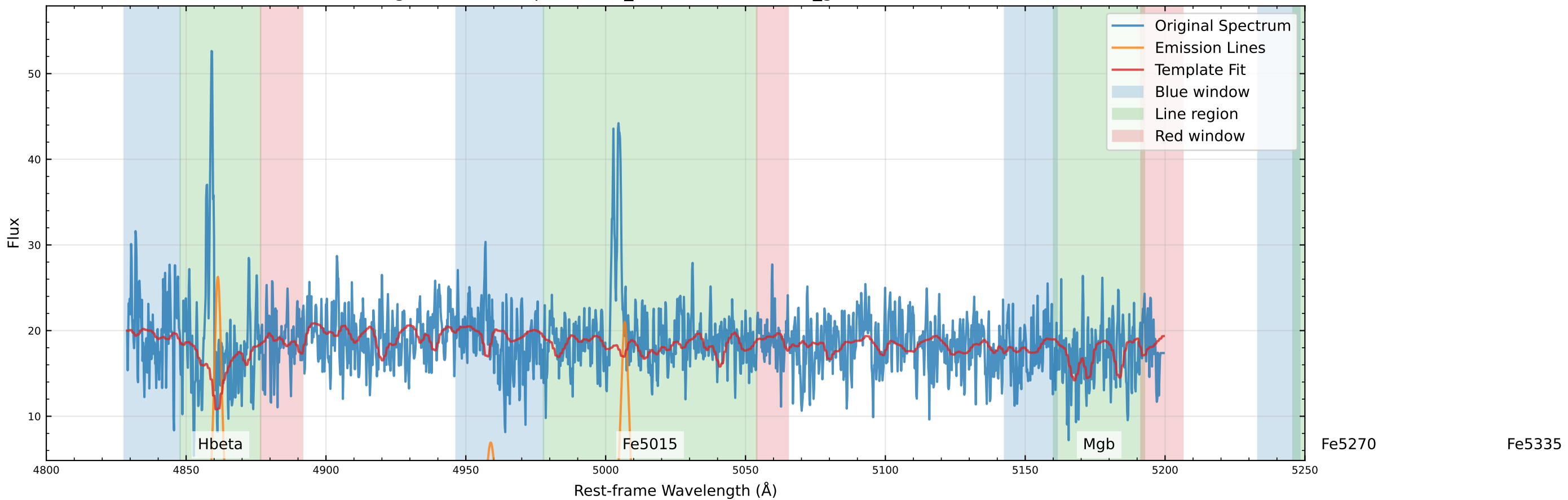
Original Data Comparison (v_star=-217.9 km/s, v_gas=-158.7 km/s)
