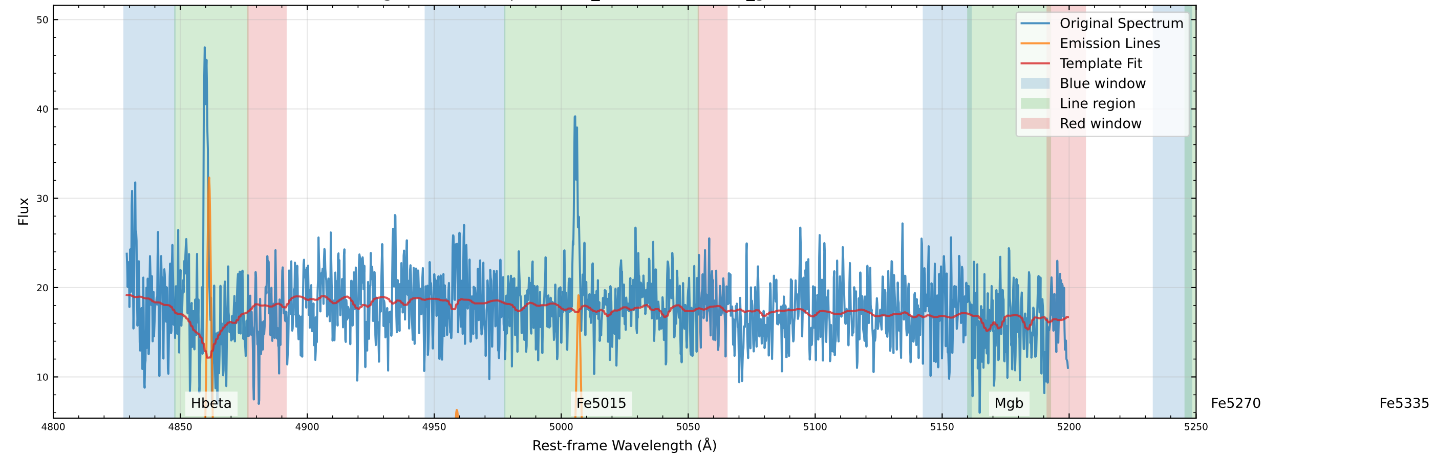
Original Data Comparison (v_star=40.6 km/s, v_gas=-73.5 km/s)
