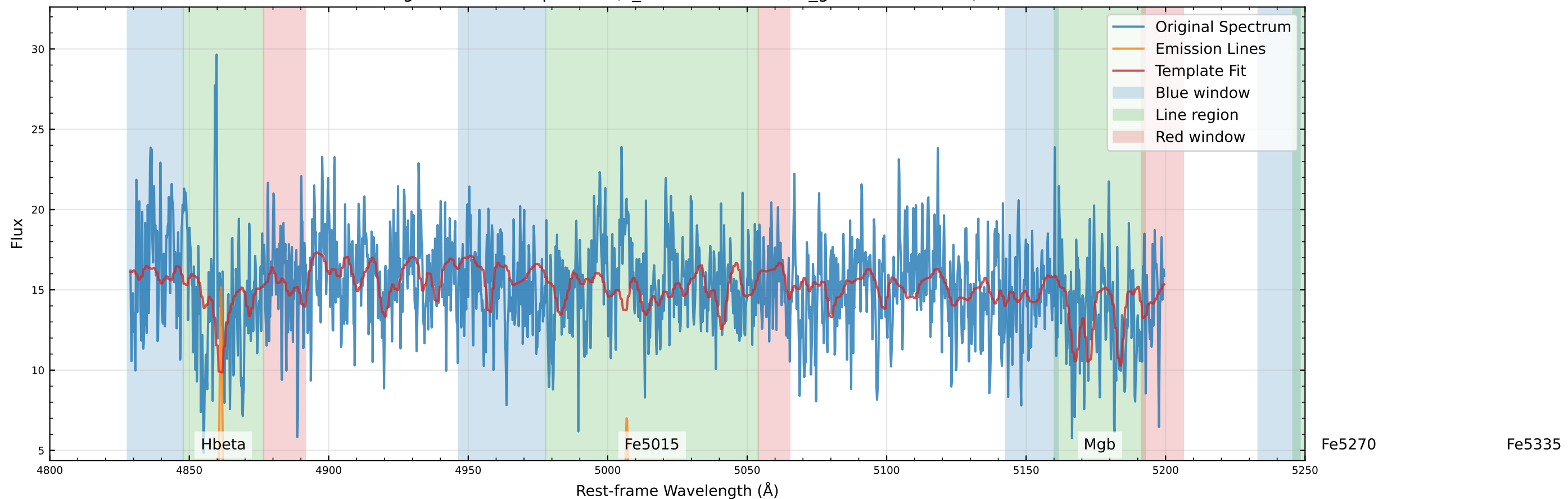
Original Data Comparison (v_star=-72.9 km/s, v_gas=-112.1 km/s)
