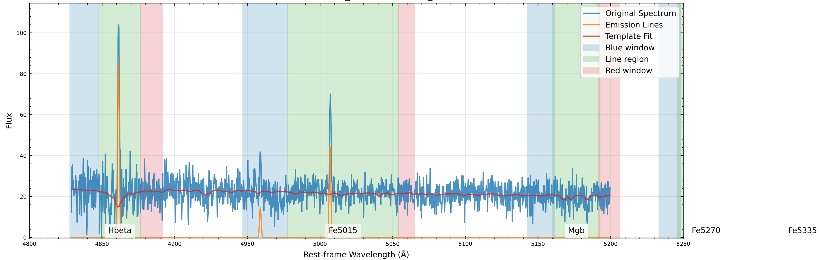
Original Data Comparison (v_star=3.1 km/s, v_gas=5.8 km/s)
