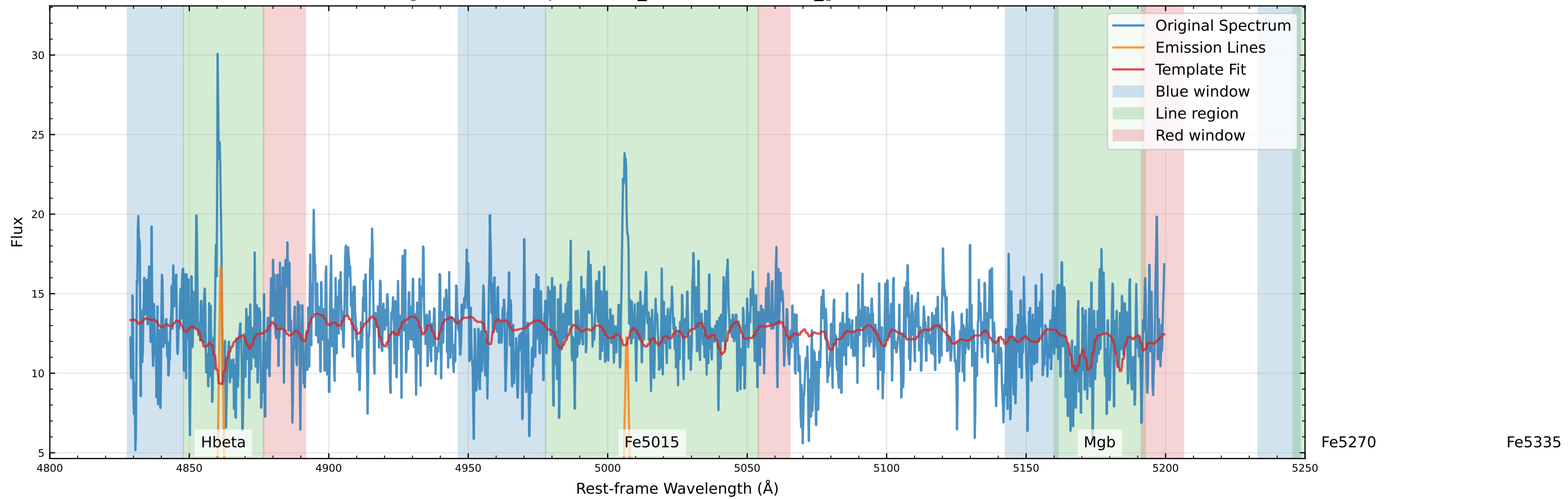
Original Data Comparison ( v_{\text{star}}=-59.3 km/s, v_{\text{gas}}=-46.8 km/s)
