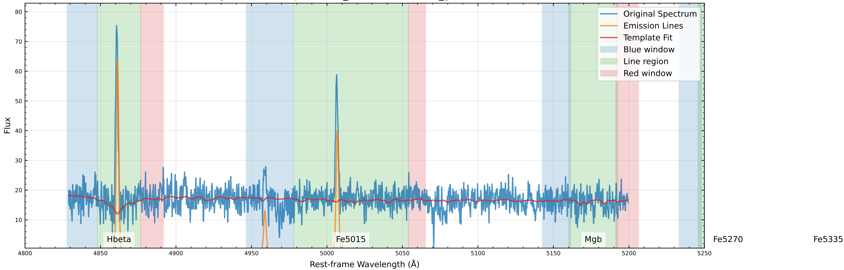
Original Data Comparison (v_star=-71.7 km/s, v_gas=-29.3 km/s)
