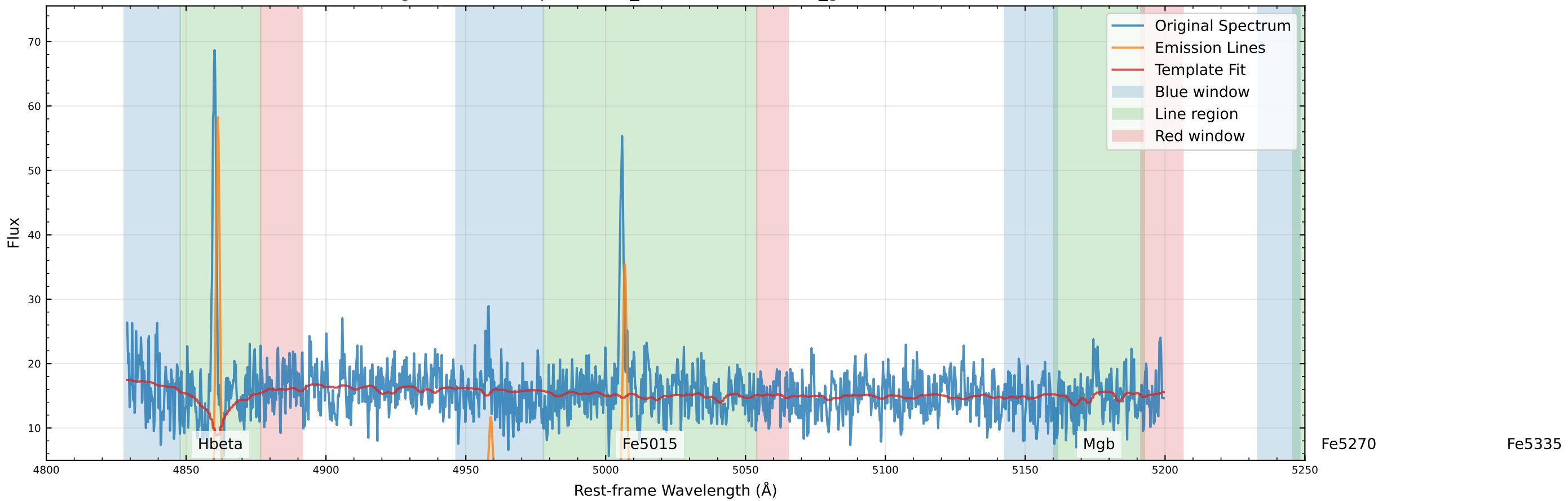
Original Data Comparison (v_star=-100.2 km/s, v_gas=-73.1 km/s)
