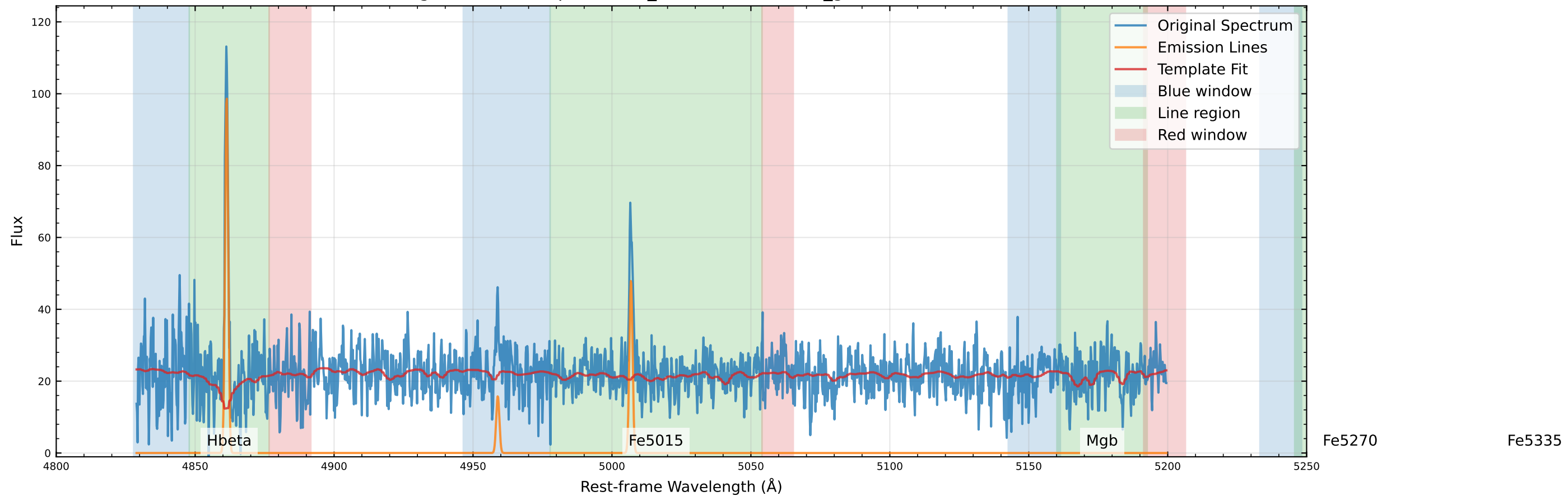
Original Data Comparison (v_star=-21.6 km/s, v_gas=-3.5 km/s)
