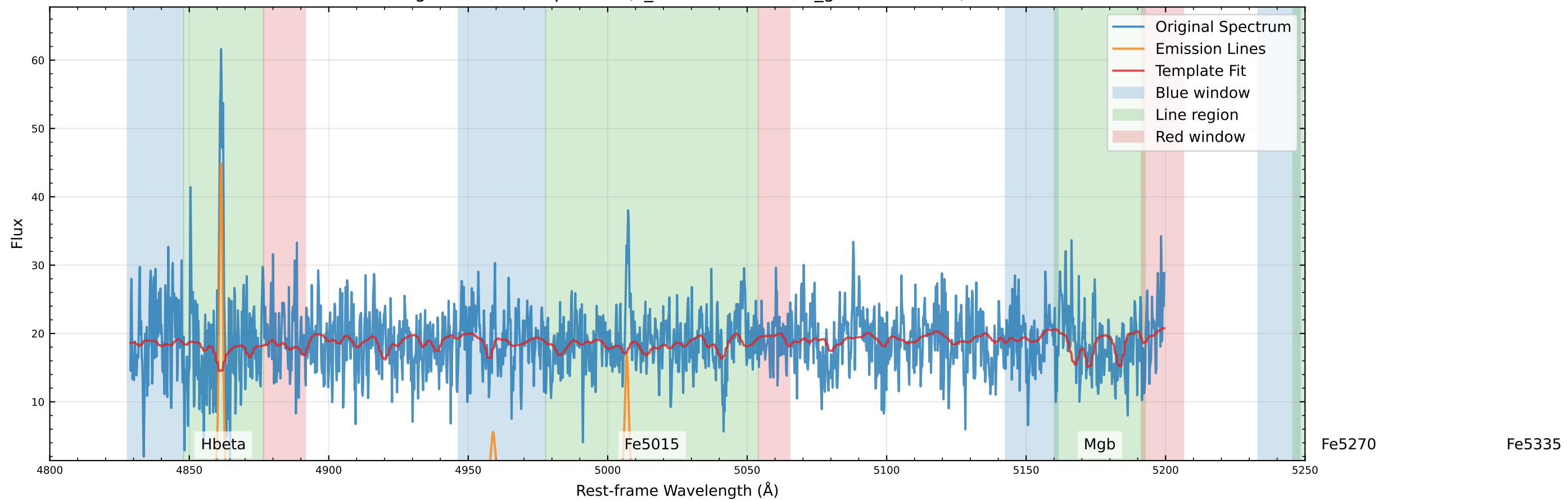
Original Data Comparison (v_star=15.8 km/s, v_gas=11.3 km/s)
