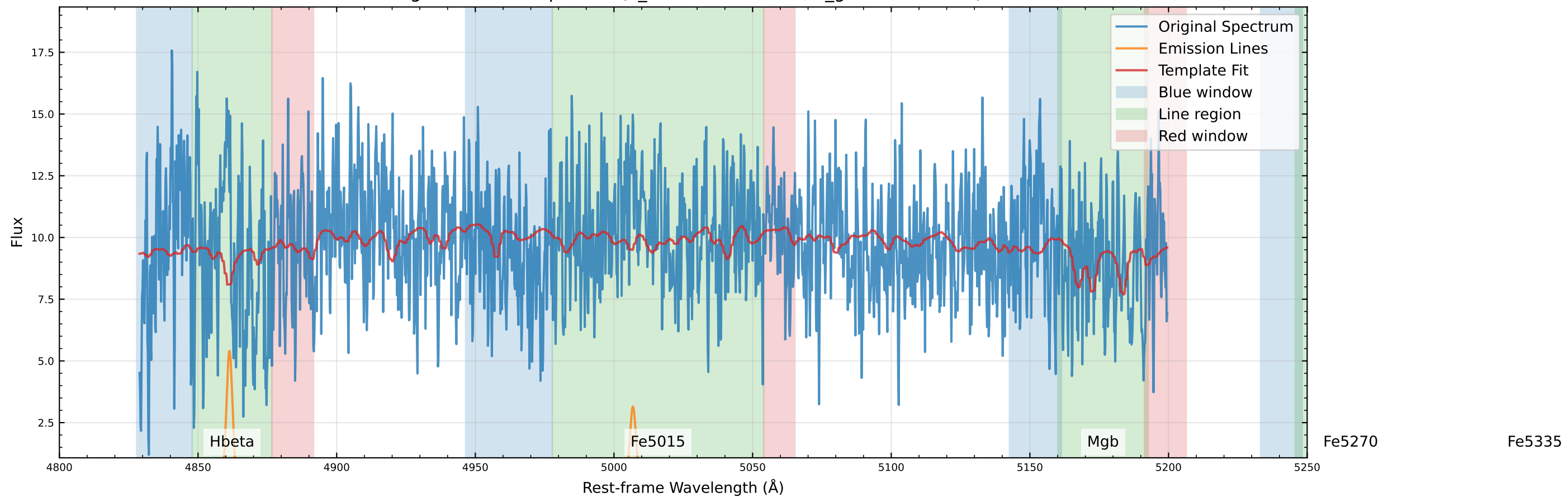
Original Data Comparison ( v_{\text{star}}=-201.6 km/s, v_{\text{gas}}=-65.4 km/s)
