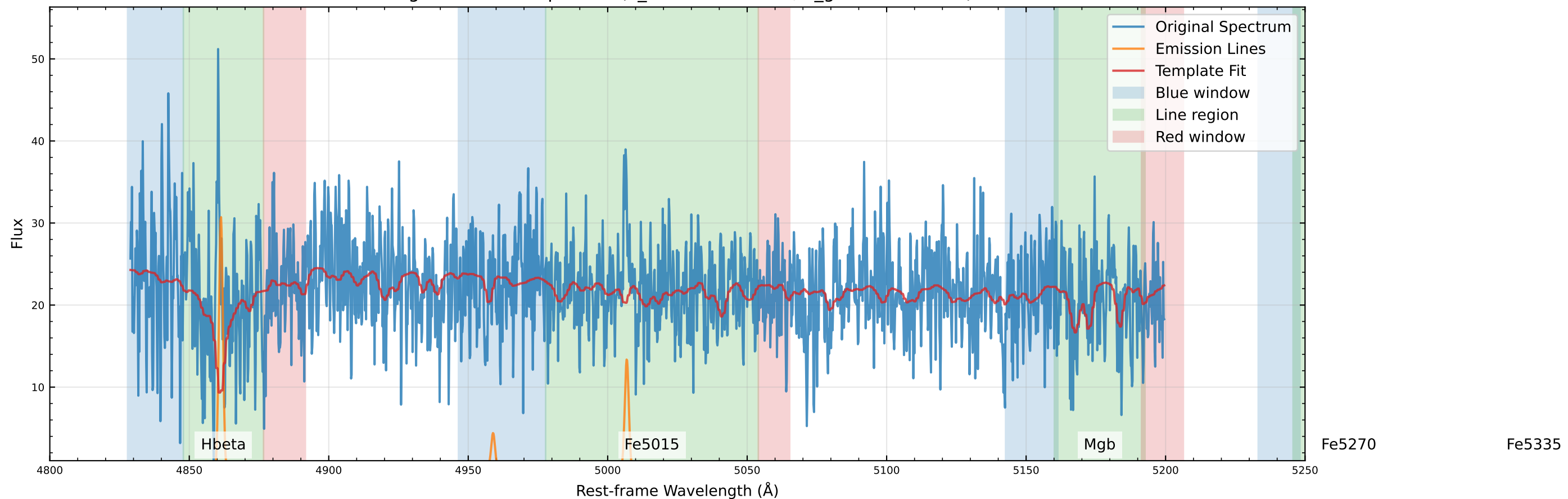
Original Data Comparison (v_star=-19.5 km/s, v_gas=-50.7 km/s)
