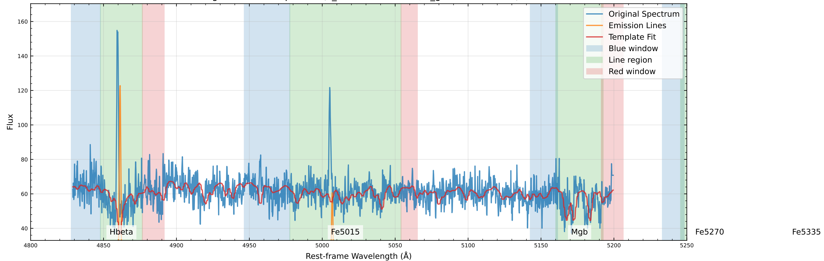
Original Data Comparison (v_star=-108.2 km/s, v_gas=-103.0 km/s)
