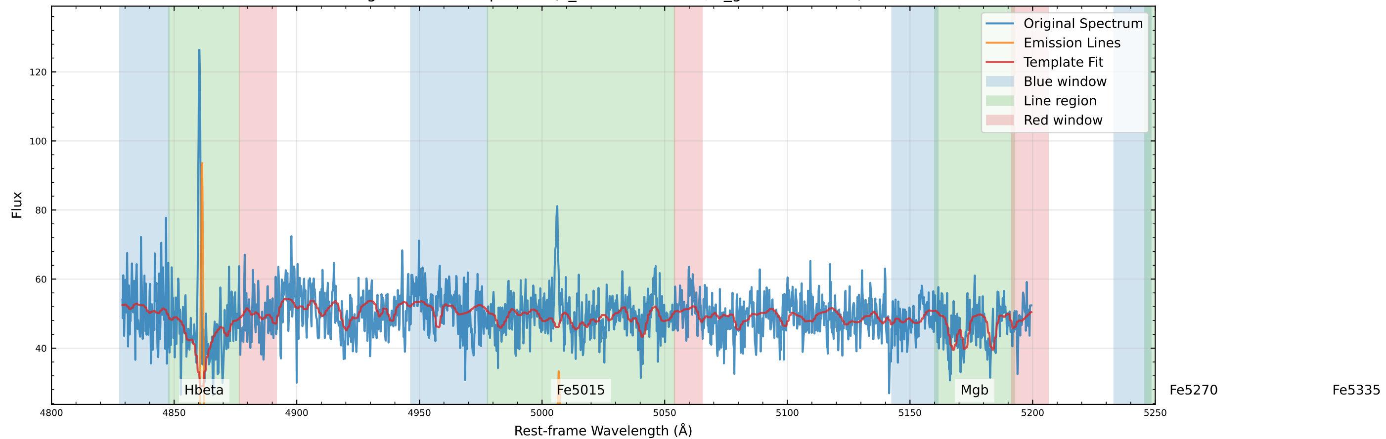
Original Data Comparison (v_star=-64.8 km/s, v_gas=-62.6 km/s)
