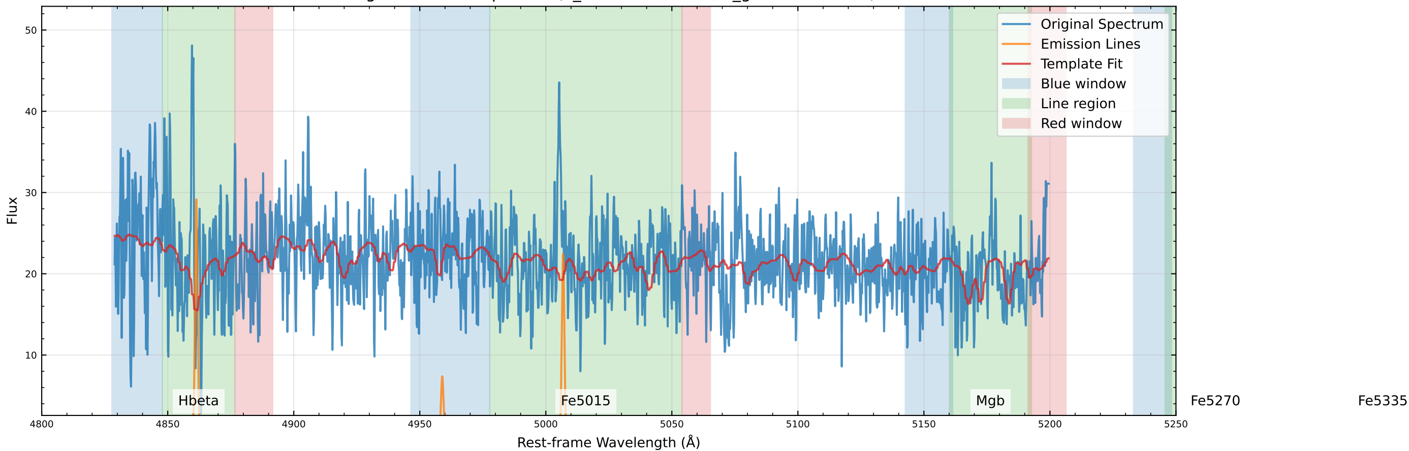
Original Data Comparison (v_star=-99.4 km/s, v_gas=-94.1 km/s)
