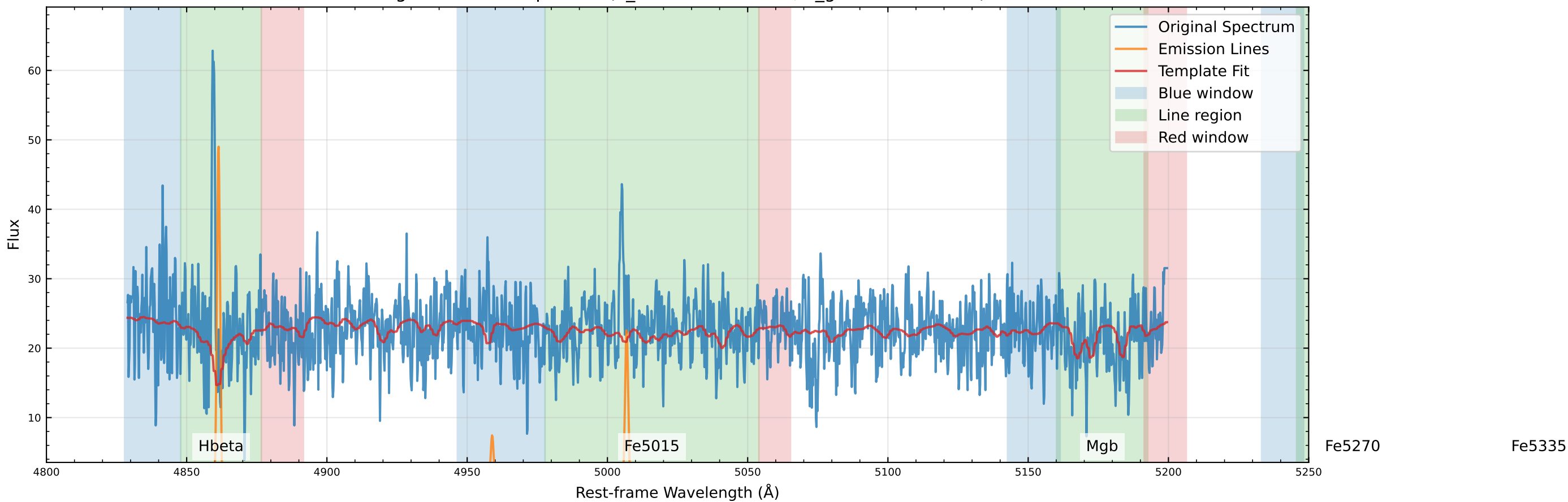
Original Data Comparison (v_star=-104.8 km/s, v_gas=-112.5 km/s)
