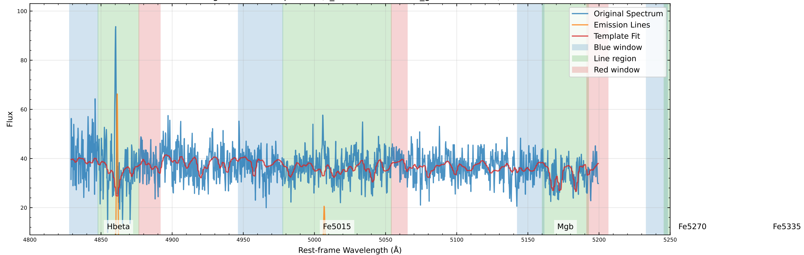
Original Data Comparison (v_star=-61.5 km/s, v_gas=-67.7 km/s)
