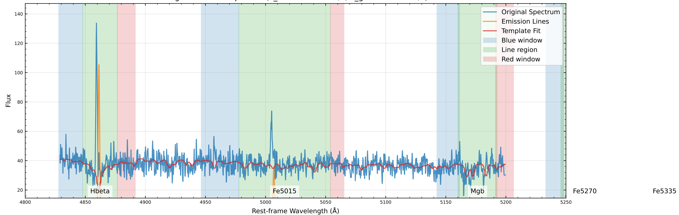
Original Data Comparison (v_star=-102.3 km/s, v_gas=-120.1 km/s)
