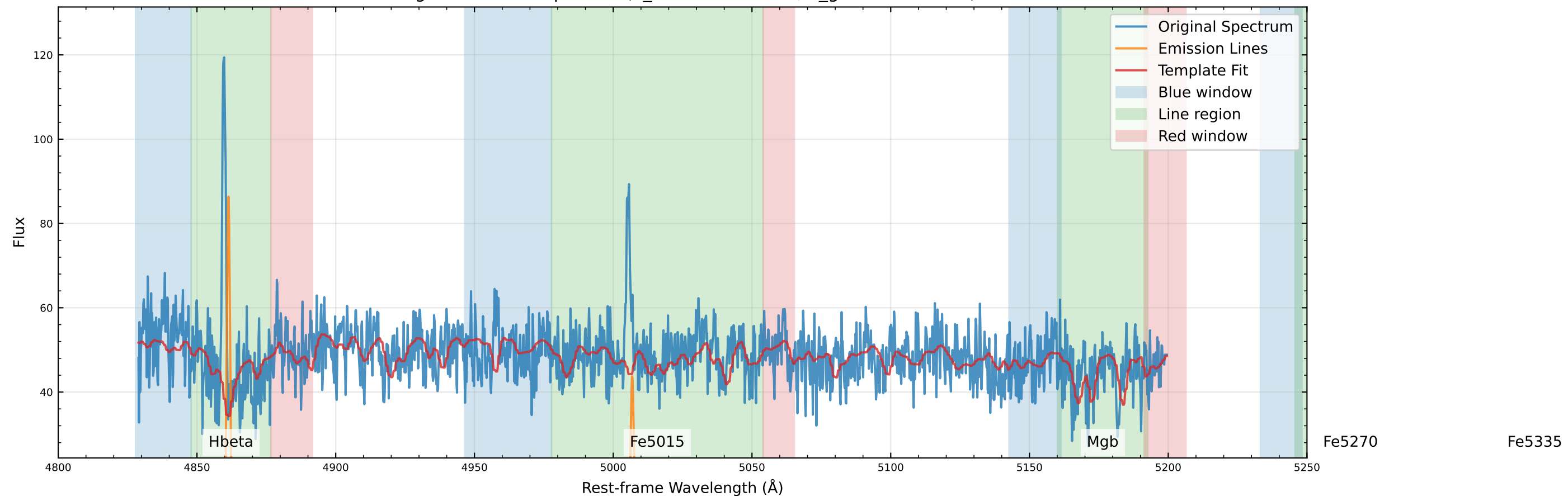
Original Data Comparison (v_star=-87.4 km/s, v_gas=-96.9 km/s)
