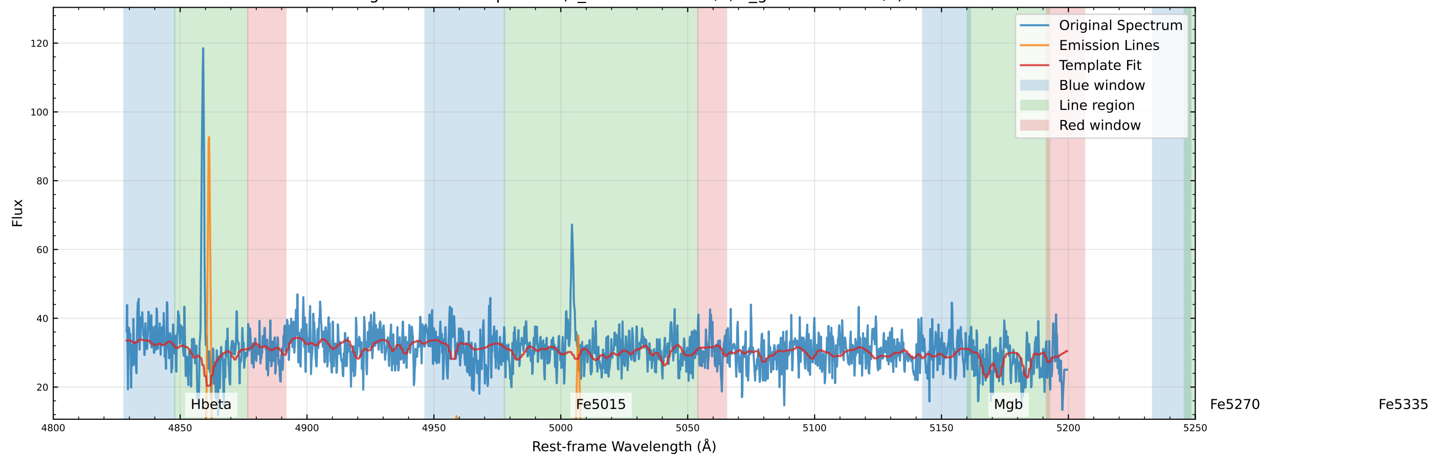
Original Data Comparison (v_star=-134.0 km/s, v_gas=-144.8 km/s)
