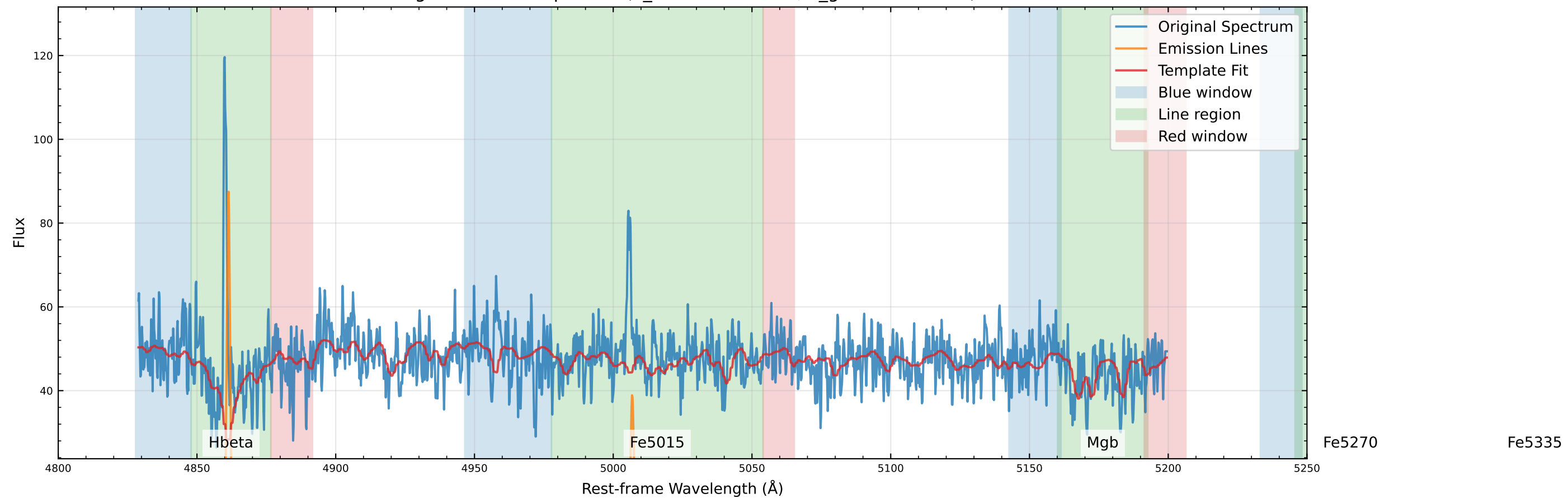
Original Data Comparison (v_star=-71.6 km/s, v_gas=-73.4 km/s)
