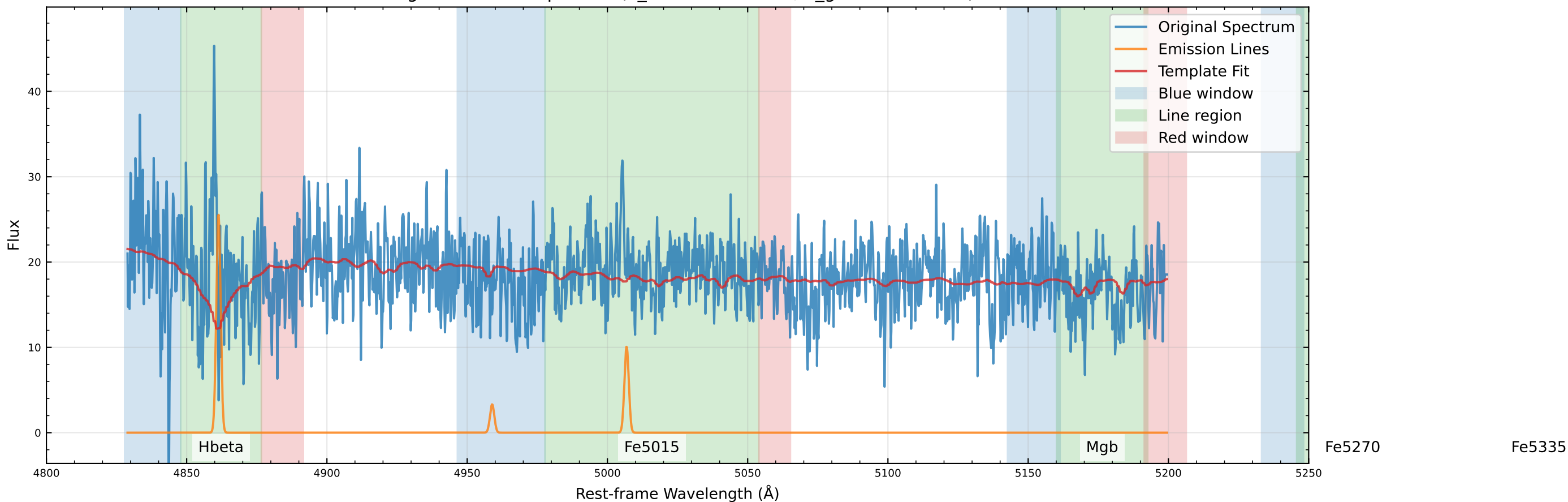
Original Data Comparison (v_star=-93.5 km/s, v_gas=-99.7 km/s)
