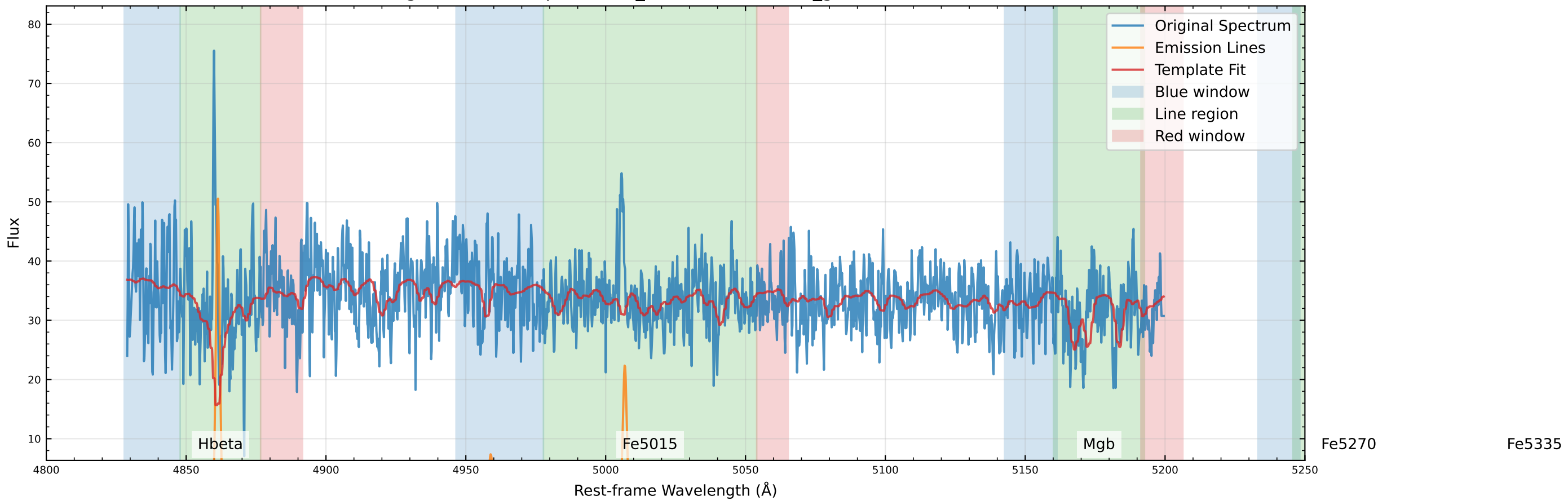
Original Data Comparison (v_star=-89.3 km/s, v_gas=-74.9 km/s)
